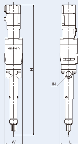
Type ND dimensional outline drawing
